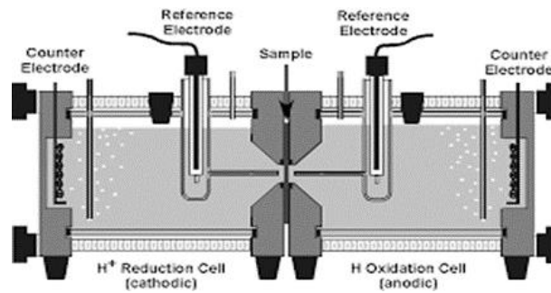
Figure 28: General scheme of the hydrogen permeation (DEVANATHAN) cell
