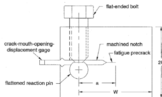
Figure 17: Typical geometry of compact specimen (CT) for fracture toughness test according to ISO 1114-4
