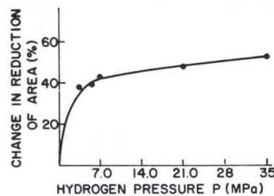
Figure 16: Influence of hydrogen pressure on reduction in area losses for steel similar to X42. Tensile tests with double notched grade X42 specimens were used [105]
