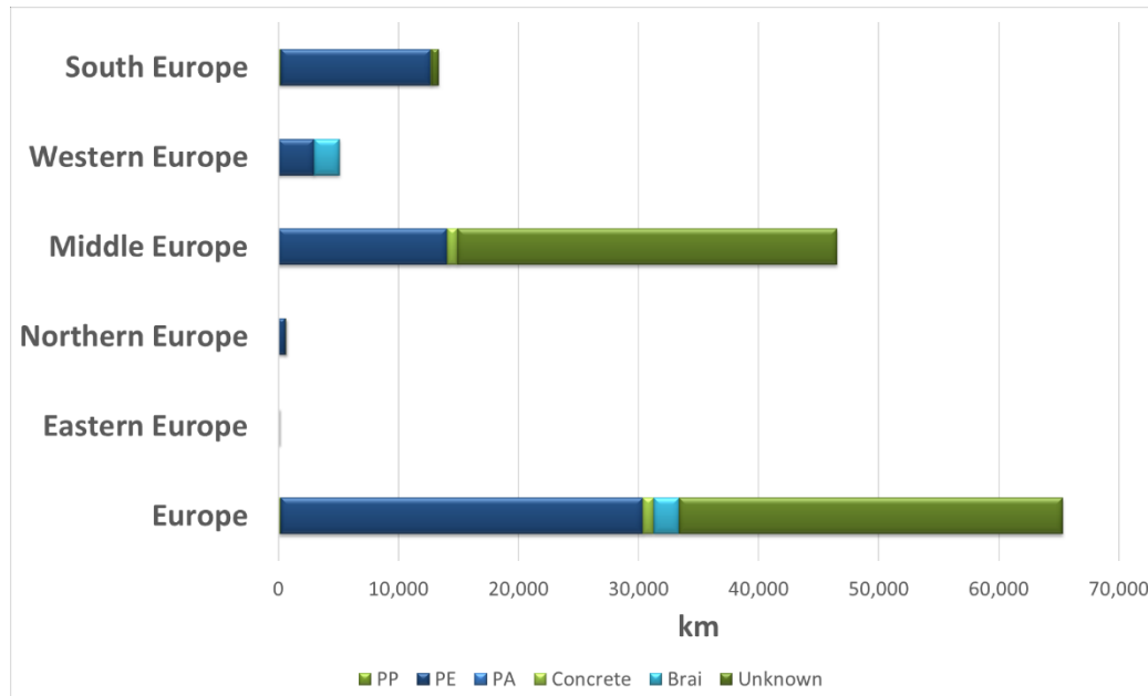
Figure 6. Outer coating materials used in the European transmission grid pipelines.
