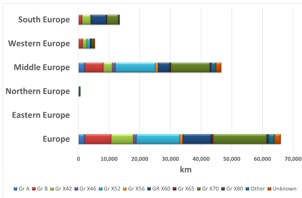
Figure 3. Distribution of the steel quality for the different clusters studied.
