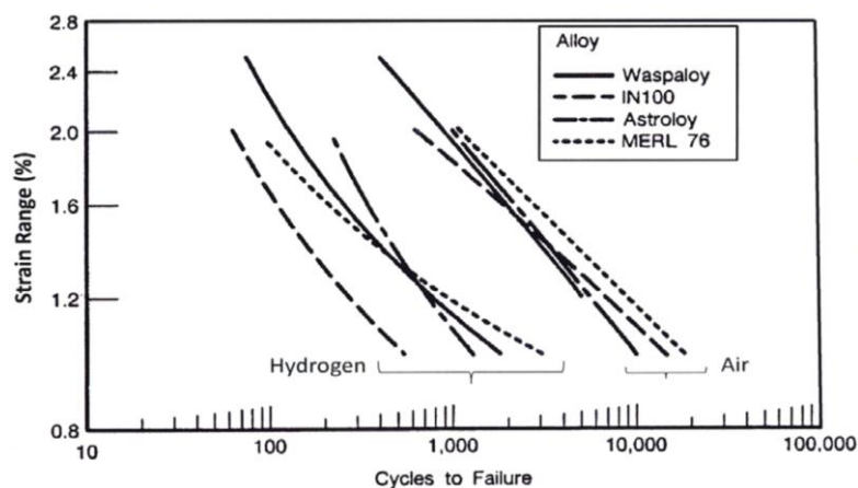
Figure 23: Effect of hydrogen on strain controlled LCF of several superalloys [106]
