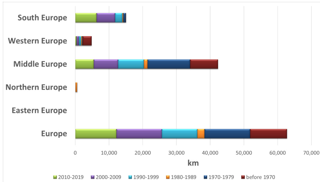
Figure 8. Installation period of pipelines in the European transmission gas grid
