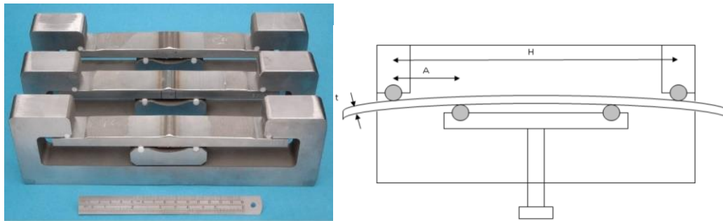
Figure 27: Four-point bend testing of welded specimens
