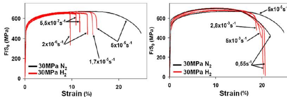
Figure 15: Tensile tests for API X80 steel tested in 30MPa of H 2 or N 2 gas for various strain rates [103]
