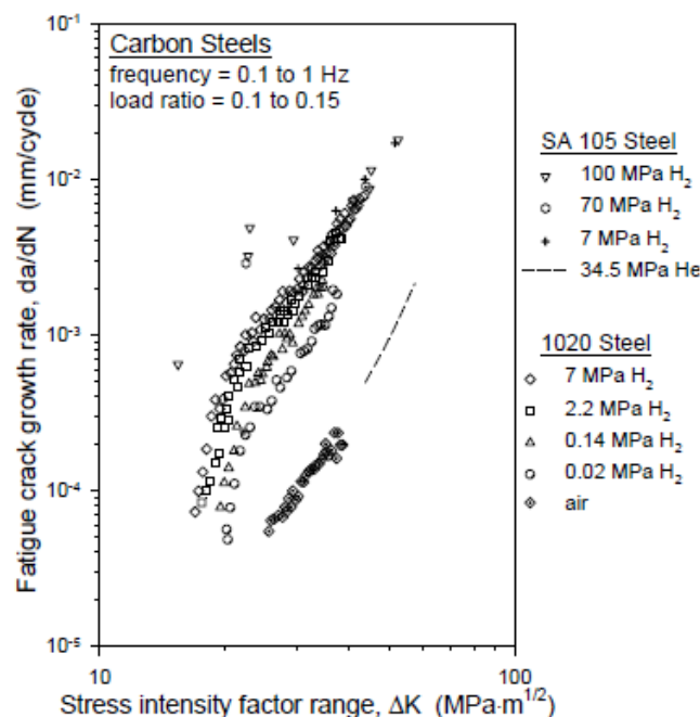
Figure 21: Effect of H_2 gas pressure on fatigue crack growth rate vs stress-intensity factor range relationships for carbon steels. Fatigue crack growth rate data in air or helium gas are included for comparison [104]
