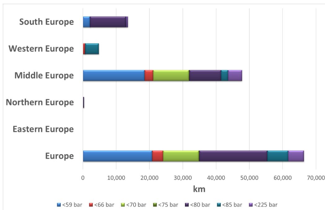
Figure 5. MOP of the transmission European grid pipelines
