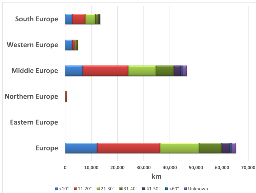
Figure 4. Diameter of the European transmission grid pipelines
