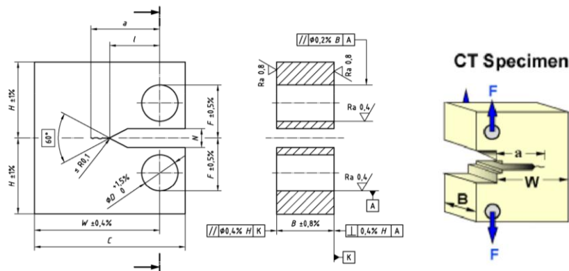
Figure 17: Typical geometry of compact specimen (CT) for fracture toughness test according to ISO 1114-4
