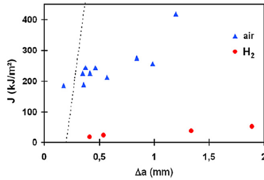
Figure 19: Fracture toughness results realized on x80 CT specimens in H 2 gas at 30 MPa and in air [103]
