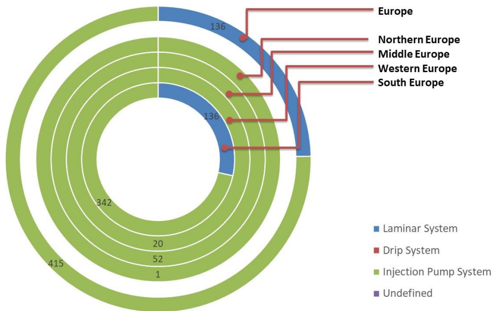
Figure 11. Odorization systems used in the European transmission grid.
