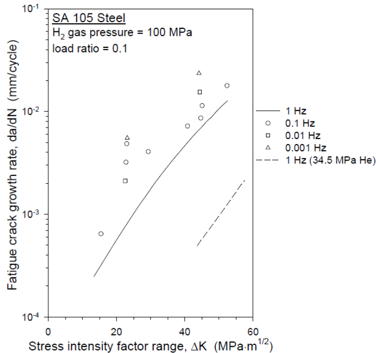
Figure 22: Effect of load cycle frequency on fatigue crack growth rate vs stress intensity factor range relationships for SA 105 steel in H 2 gas. Fatigue crack growth rate data in helium gas are included for comparison [104]
