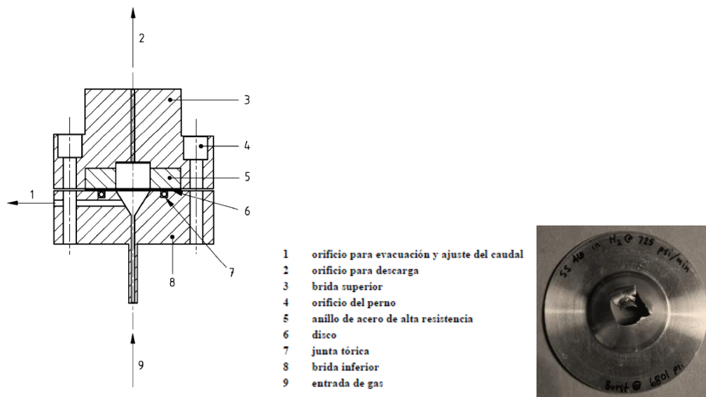
Figure 24: Disk testing method indicated in standard ISO 11114-4-Method A
