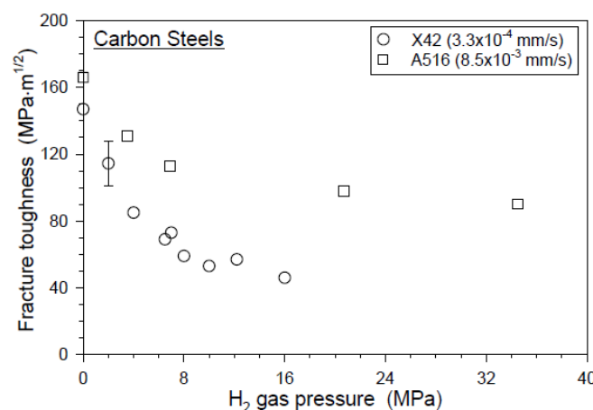
Figure 20: Effect of H 2 gas pressure on fracture toughness for carbon steels grade X42 and A516 [105]
