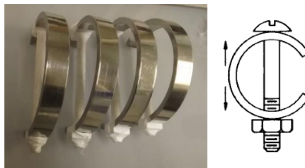
Figure 26: C-ring specimens (constant strain)
