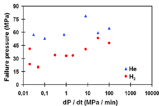
Figure 25: Disk pressure test results realized on X80 specimens [103]
