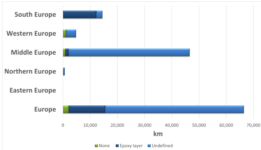
Figure 7. Inner coating materials used in the European transmission grid pipelines.
